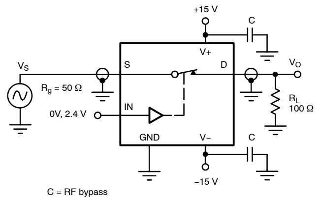
FIGURE 6. Insertion Loss
