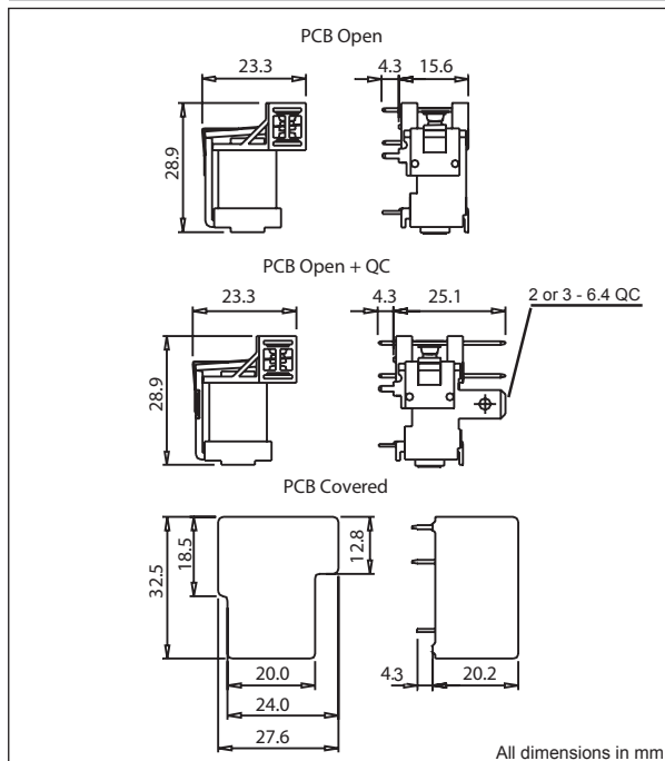
Overall Dimensions - PCB Relays
