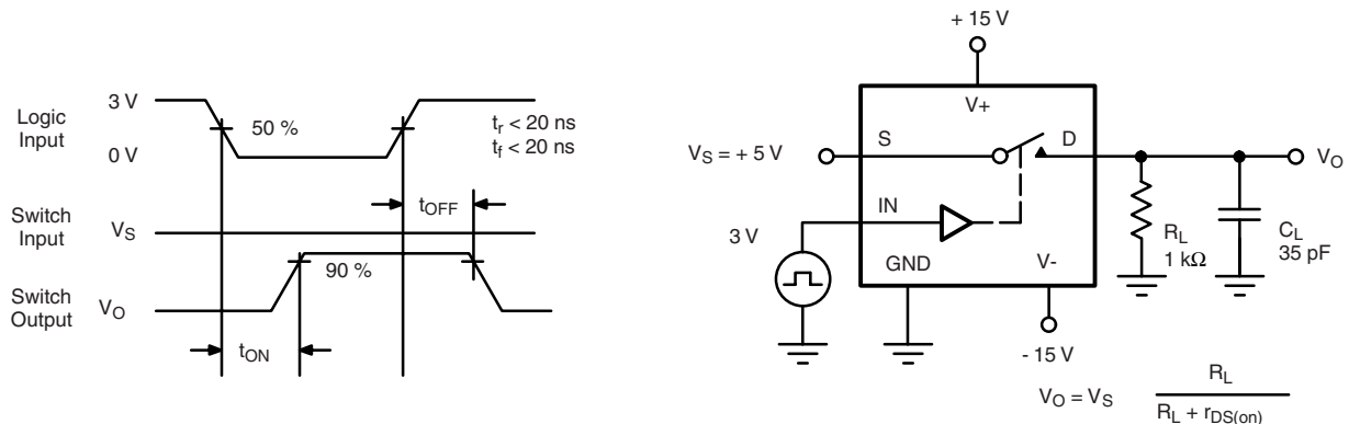
Figure 2. Switching Time
