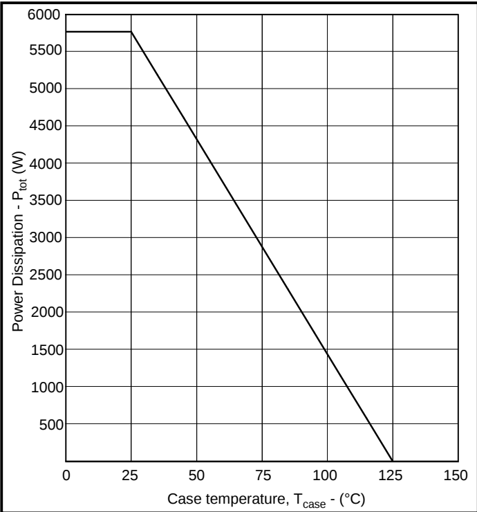
Fig. 5 Power dissipation
