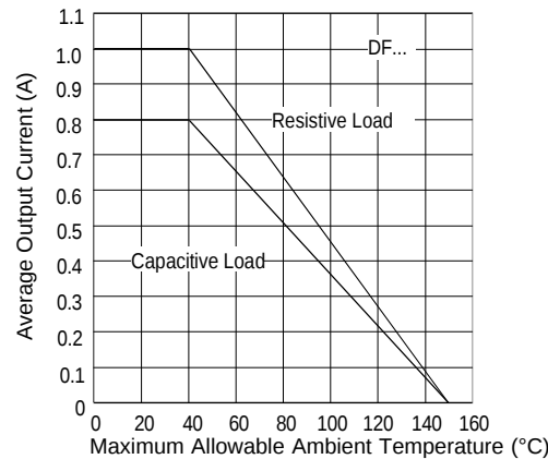
Fig. 3 - Current Ratings
