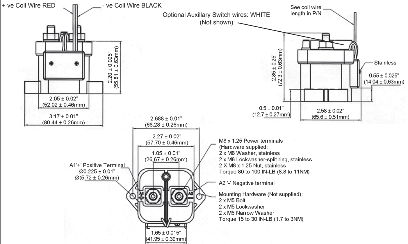
Overall Dimensions
