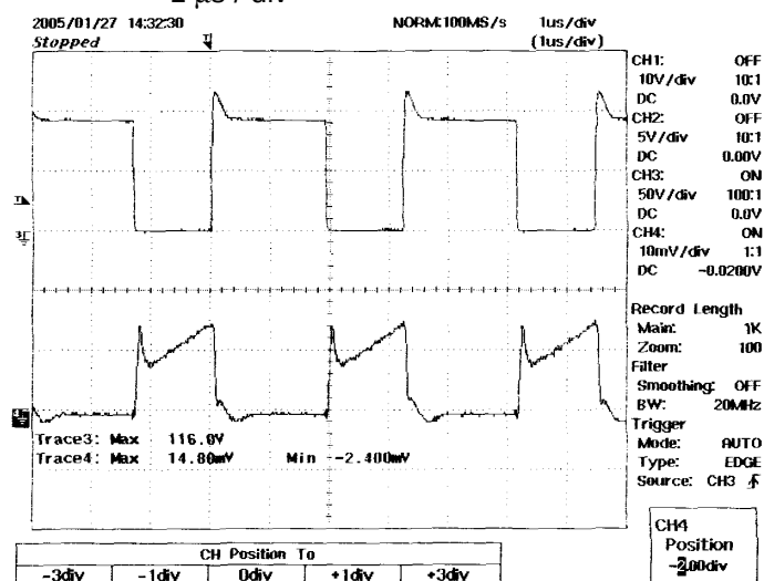
Figure 14 – 57 VDC, full load
