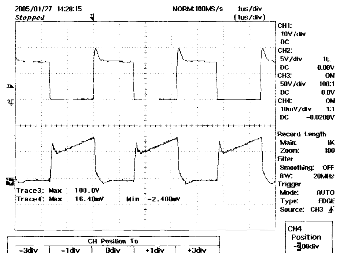
Figure 12 – 37 VDC, full load
