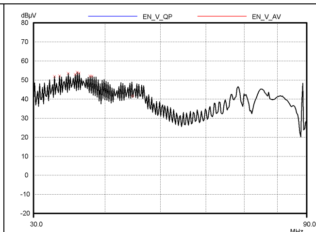
Figure 32 – Original board with DPA423 and AC-adaptor (230 VAC) – Output Floating
