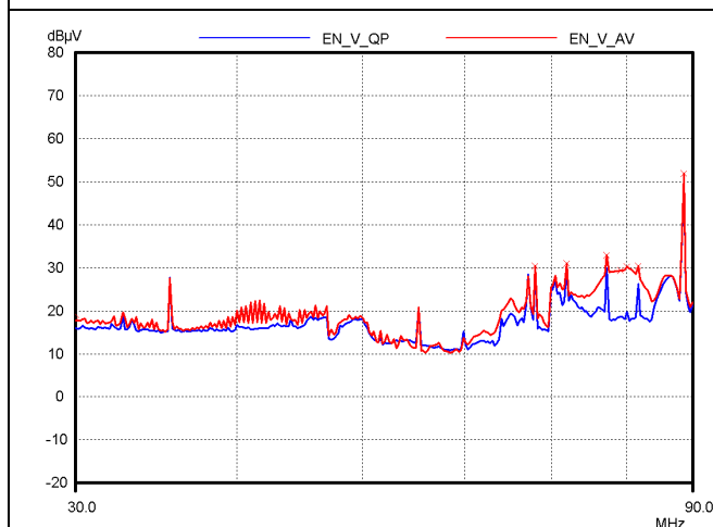
Figure 33 – New prototype board using DPA423 and AC-adaptor (230 VAC) – Output Floating
