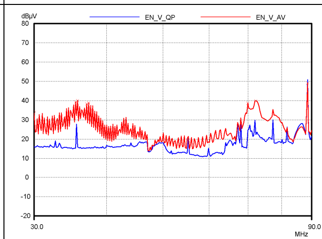
Figure 34 – New prototype board using DPA423 and AC-adaptor (230 VAC) – Output Hard Grounded
