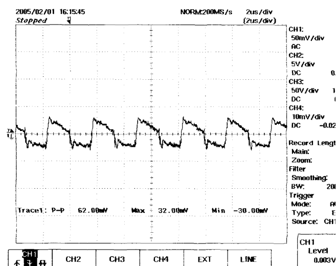
Figure 19 – 48 VDC, Full Load 5V Output Ripple, 50 mV, 2 \mu\text{s} / div
