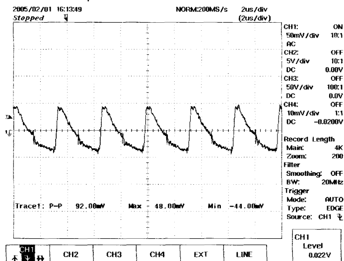
Figure 20 – 48 VDC, Full Load 12 V Output Ripple, 50 mV, 2 \mu\text{s} / div
