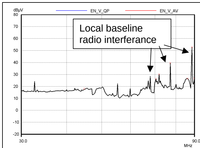
Figure 31 – Radiated no-power Baseline
