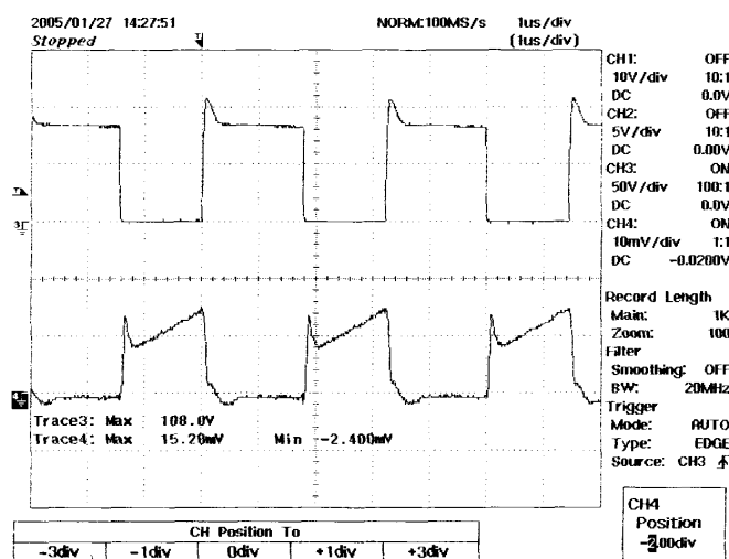
Figure 13 – 48 VDC, full load
