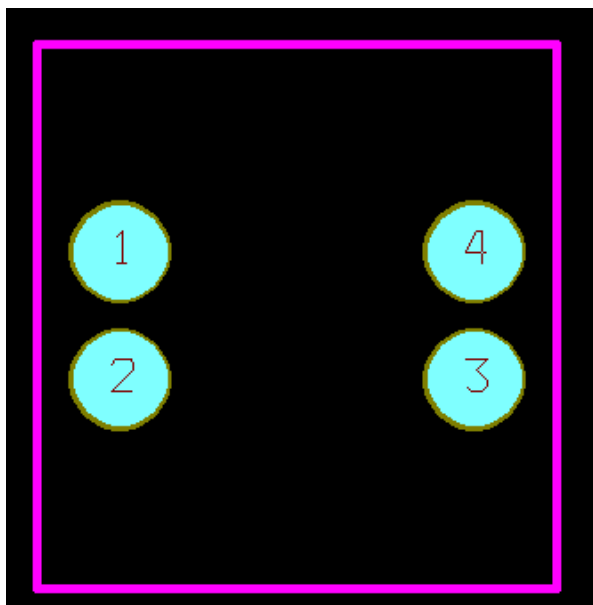
Figure 6 – Transformer Footprint – Top Side View Diagram
