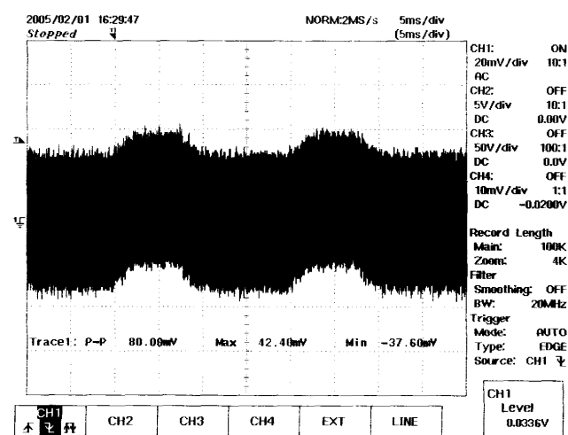
Figure 16 – 48 VDC, full load (5 V 0.16 A to 0.2 A step) 5 V Output Voltage 20 mV / Div, 10 ms / div
