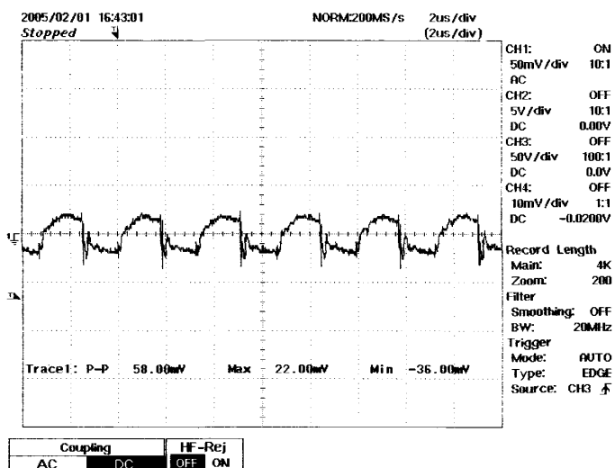
Figure 18 – 48 VDC, Full Load 3.3 V Output Ripple, 50 mV, 2 \mu\text{s} / div
