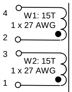
Figure 5 – Inductor Electrical Diagram
