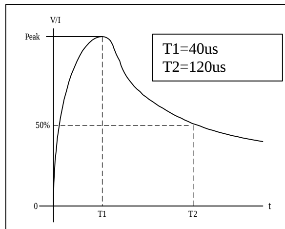
Figure 10 Current/Voltage Waveform 5A
