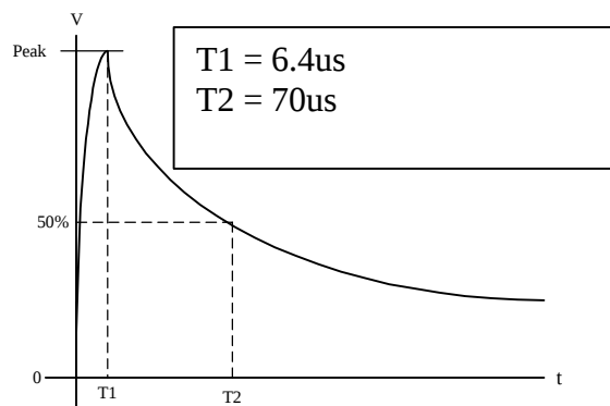
Figure 9 Voltage Waveform 4
