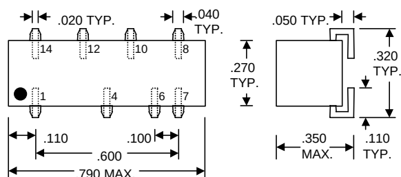
DDU4F-xxB2 (Commercial J-Lead)
