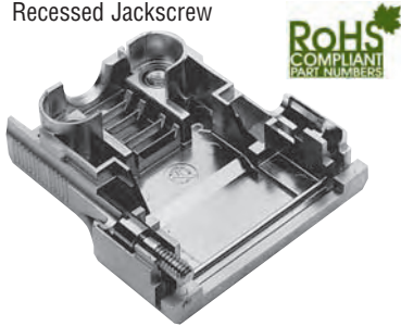
Recessed Jackscrew
