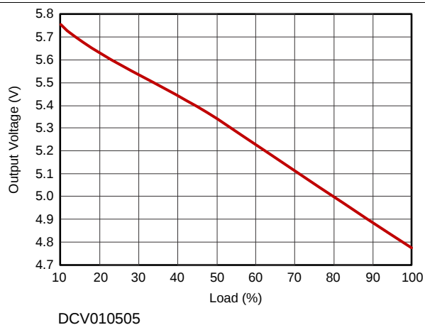
Figure 3. Load Regulation
