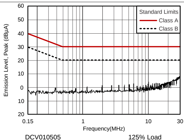
Figure 5. Conducted Emissions
