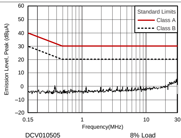
Figure 6. Conducted Emissions
