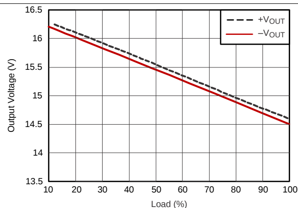
DCV012415D
