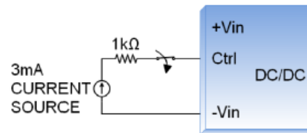
DC/DC OFF
