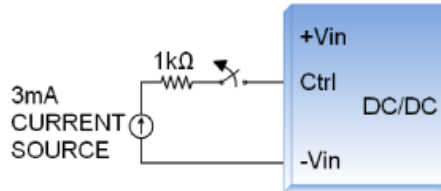
DC/DC ON
