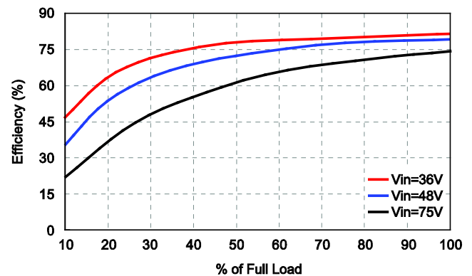
DCSD01-48S05 Efficiency vs Output Current
