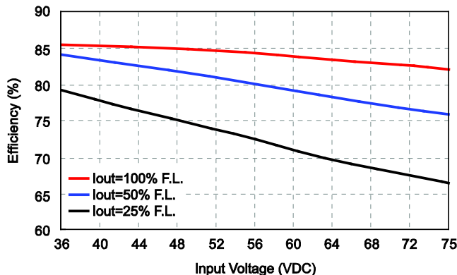
DCSD01-48S05 Efficiency vs Input Voltage
