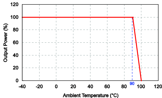
DCSD01-48S05 Derating Curve
