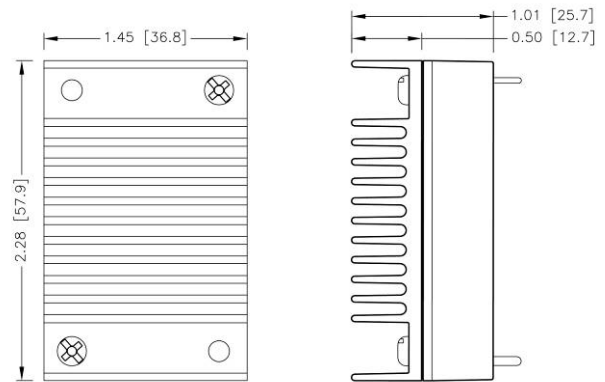
Horizontal Fin Orientation (Suffix Option: H1) 7G-0030B-F
