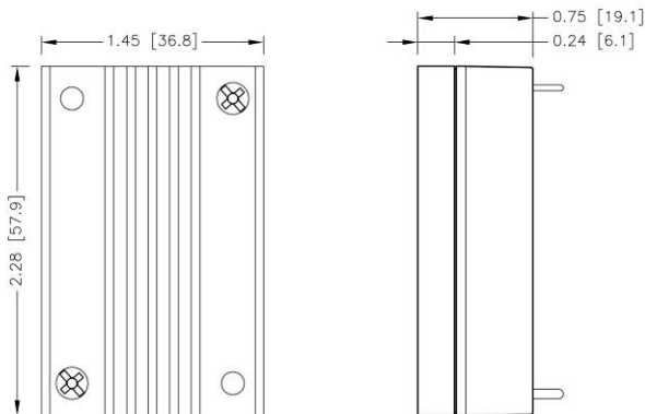
Vertical Fin Orientation (Suffix Option: H2) 7G-0031B-F
