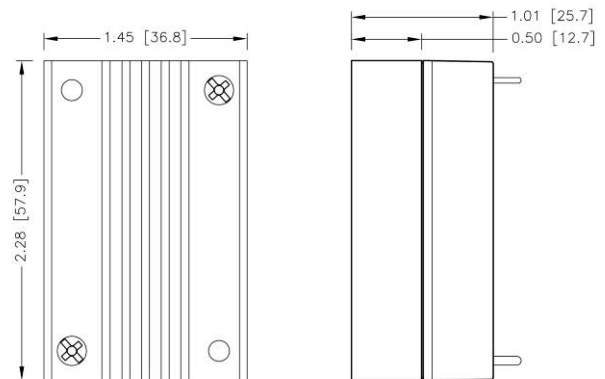
Vertical Fin Orientation (Suffix Option: H3) 7G-0032B-F
