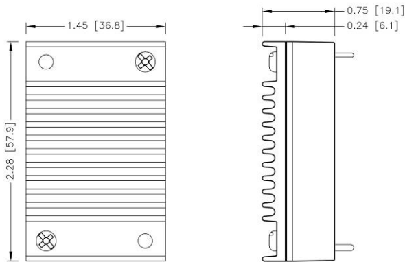
Horizontal Fin Orientation (Suffix Option: H) 7G-0029B-F
