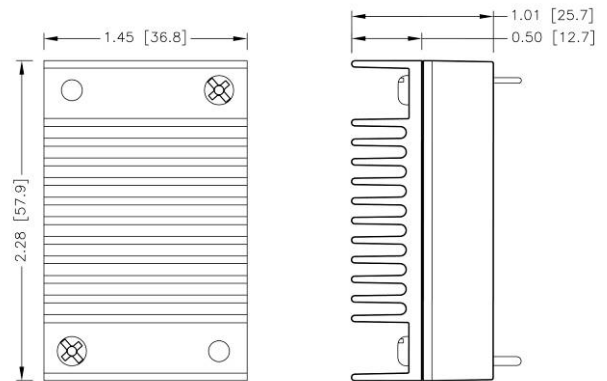
Horizontal Fin Orientation (Suffix Option: H1) 7G-0030B-F
