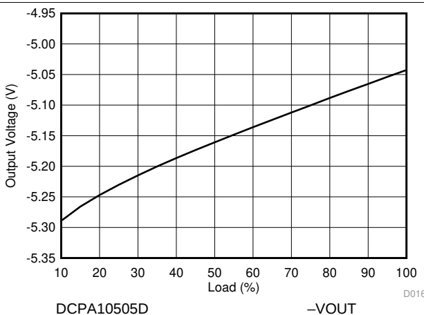
Figure 17. -VOUT Load Regulation
