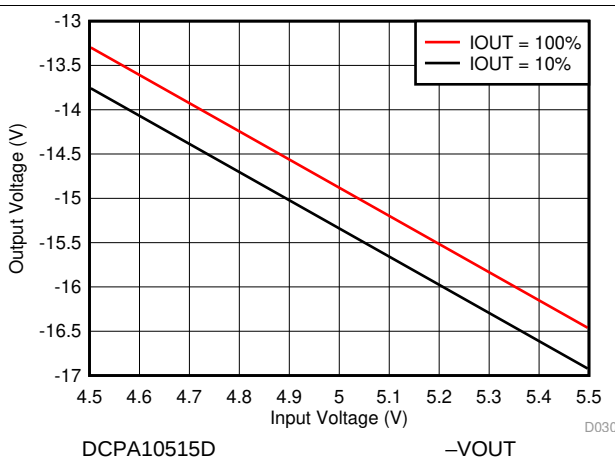
Figure 30. -VOUT Line Regulation
