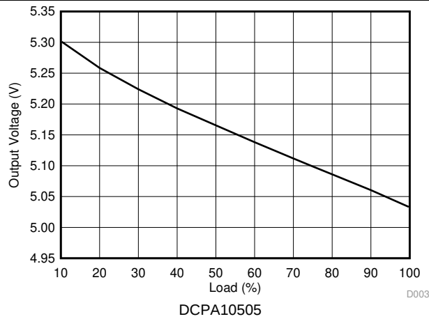
Figure 3. Load Regulation
