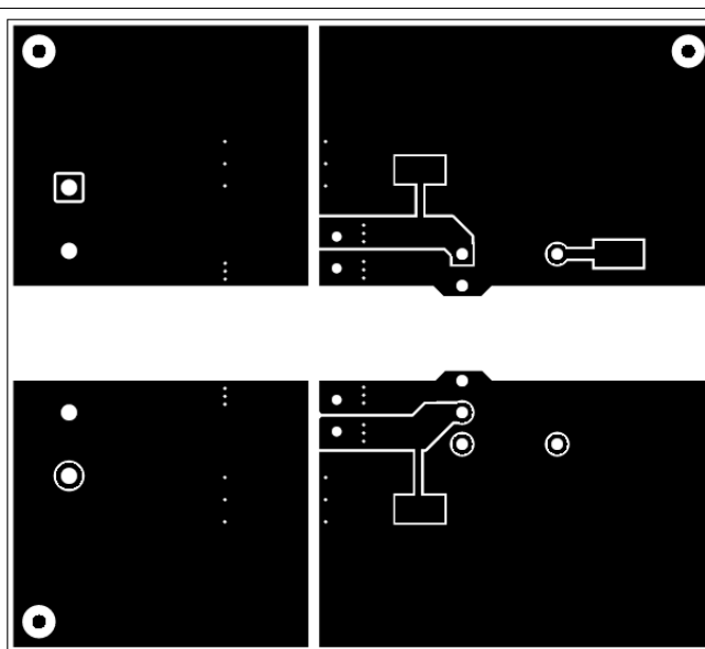
Figure 6. PWR861 Top Copper
