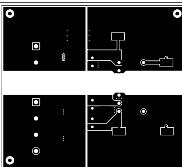
Figure 10. PWR868 Top Copper
