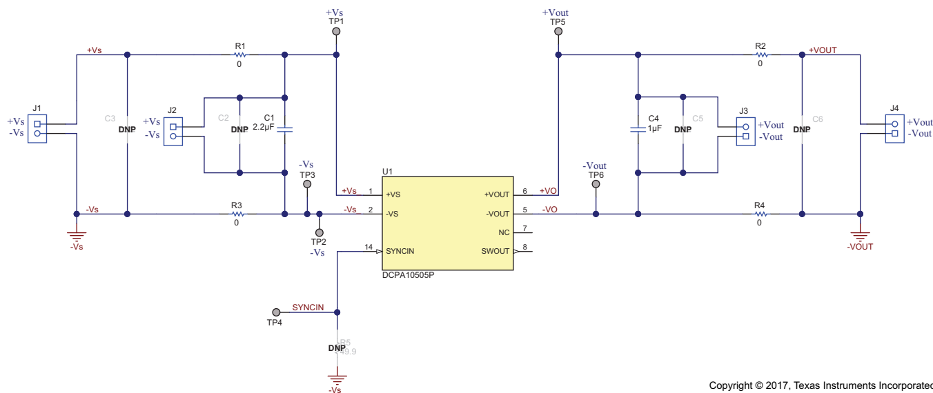
Figure 3. DCPA105xxEVM-861 Schematic
