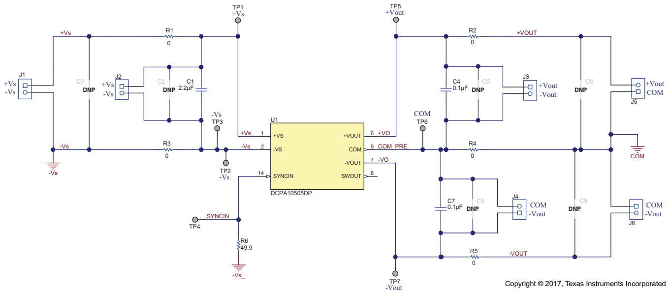
Figure 4. DCPA105xxDEVM-868 Schematic
