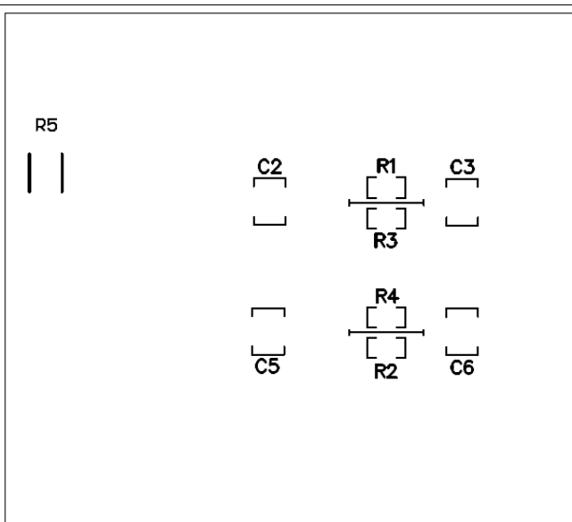
Figure 8. PWR861 Bottom Components
