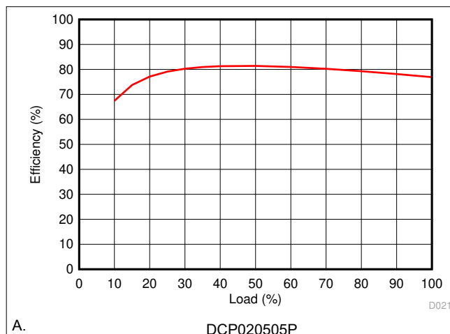
Figure 8-2. Efficiency versus Load
