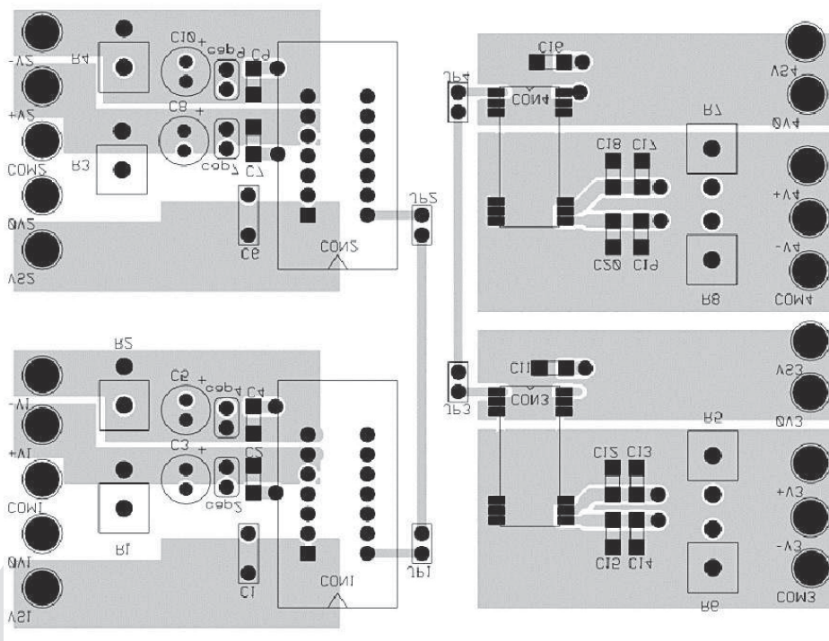
Figure 8-4. PCB Layout Example, Non-Component-Side View
