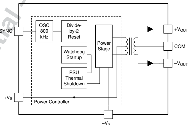
Dual Output Block Diagram
