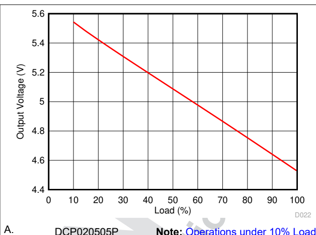
Figure 8-3. Load Regulation
