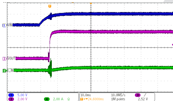
Figure 7-5. DCP020505P Start-Up at 100% Load
