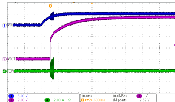
Figure 7-3. DCP020505P Start-Up at No Load
