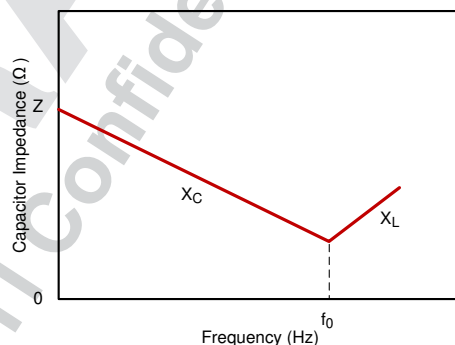
Figure 8-4. Capacitor Impedance versus Frequency
