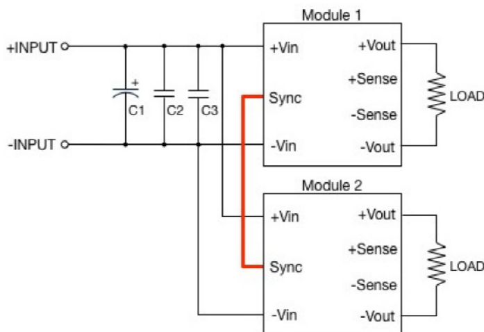
Synchronous Circuits
