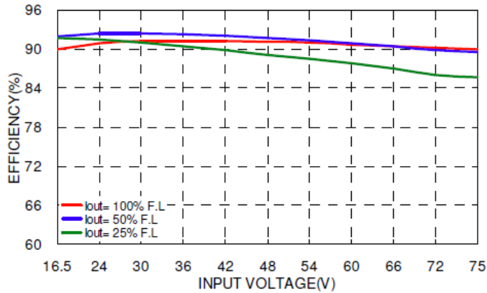
DCHBW150-48S05 Efficiency vs. Input Voltage
