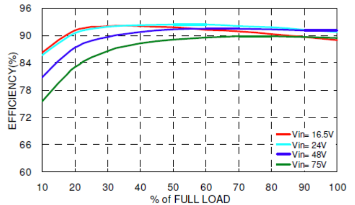
DCHBW150-48S05 Efficiency vs. Output Load
