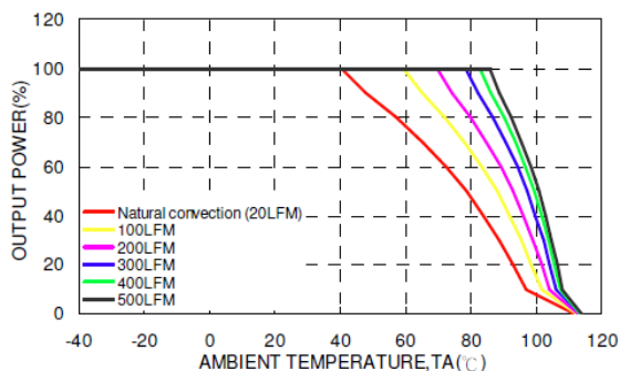
DCHBW150-48S05W Derating Curve (See Note 6) with 0.24" Height Heat-Sink
