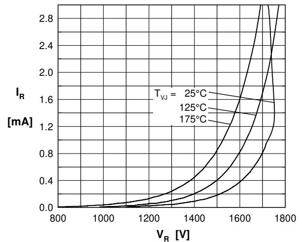
Fig. 2 Typ. reverse characteristics
