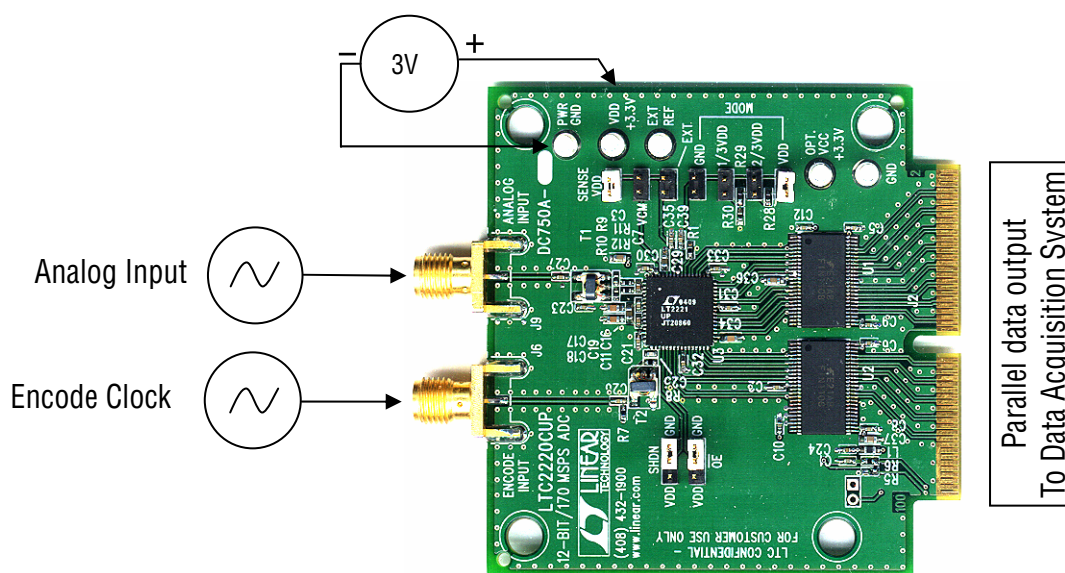
Figure 1. DC750 Setup
