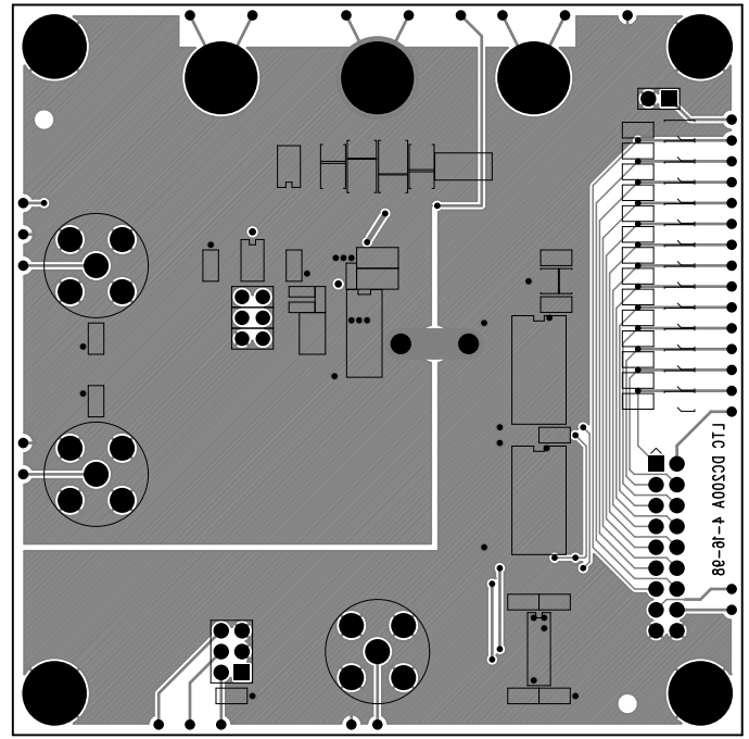
Solder Side
