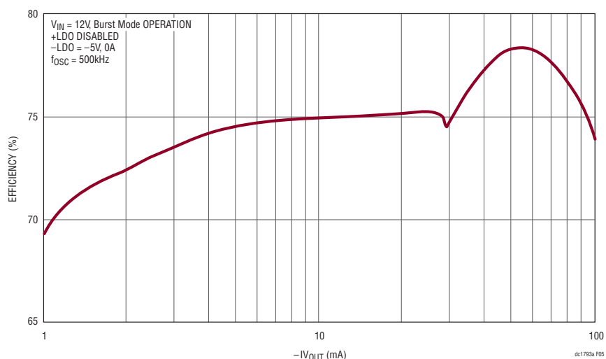
Figure 5. V IN to V OUT Burst Mode Operation Efficiency
