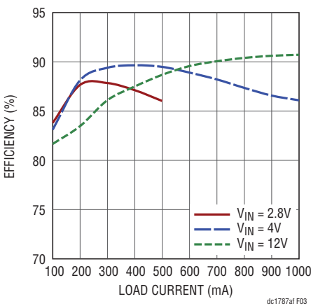
Figure 3. Efficiency Curves
