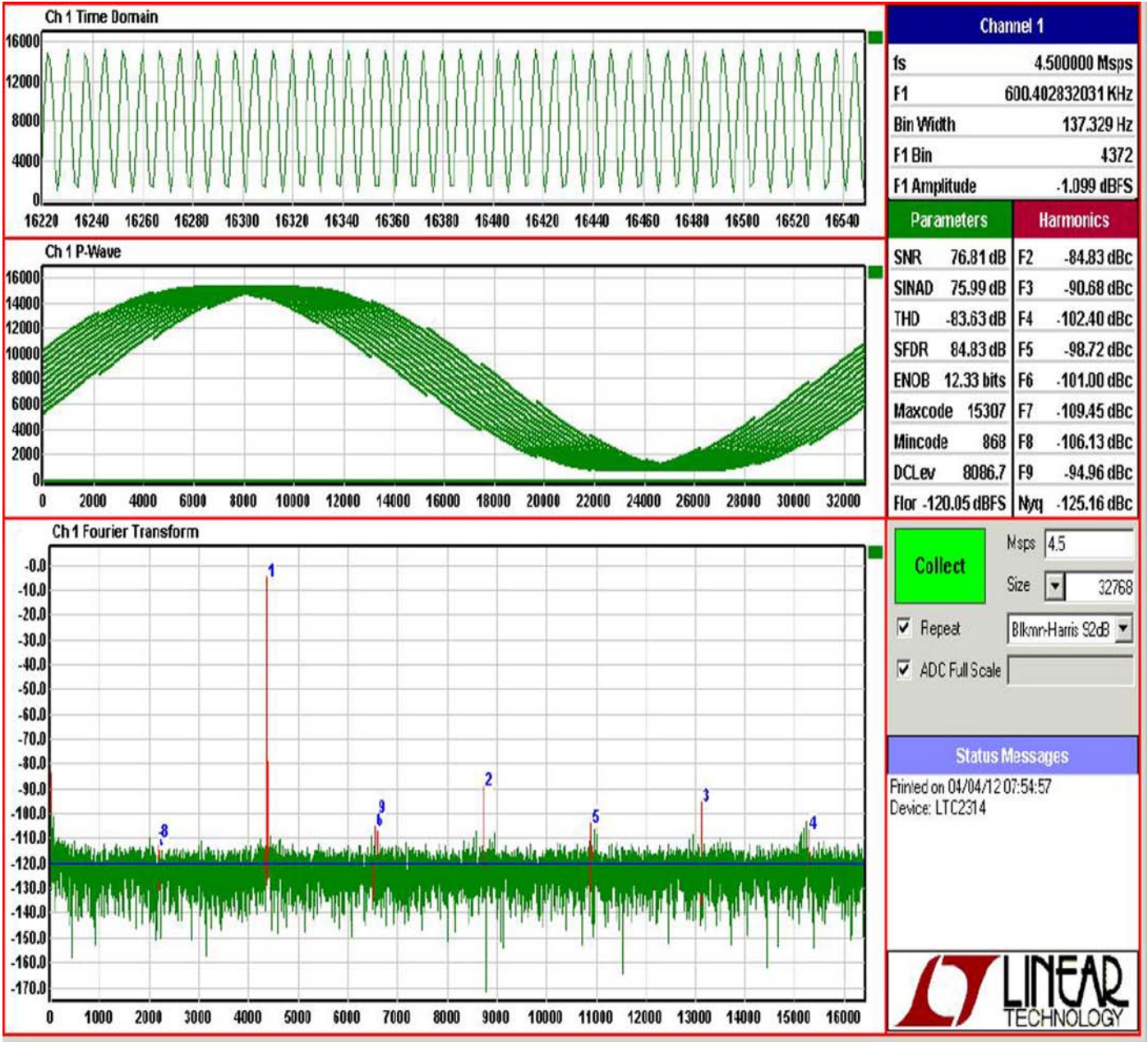
Figure 3. DC1563A-F PScope Screenshot
