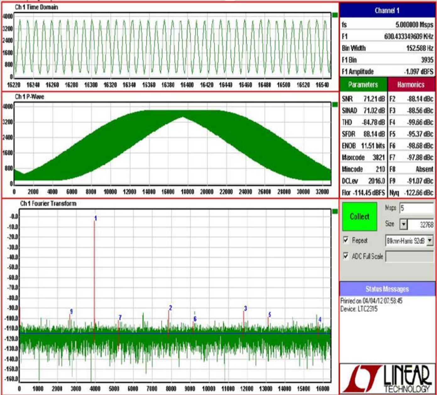
Figure 2. DC1563A-A PScope Screenshot
