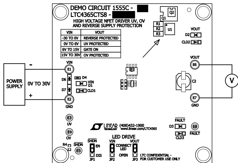
Figure 1b. Reverse Voltage Measurement
