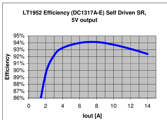
Figure 3. High efficiency of DC1317A-E allows the board to be used in thermally demanding applications
