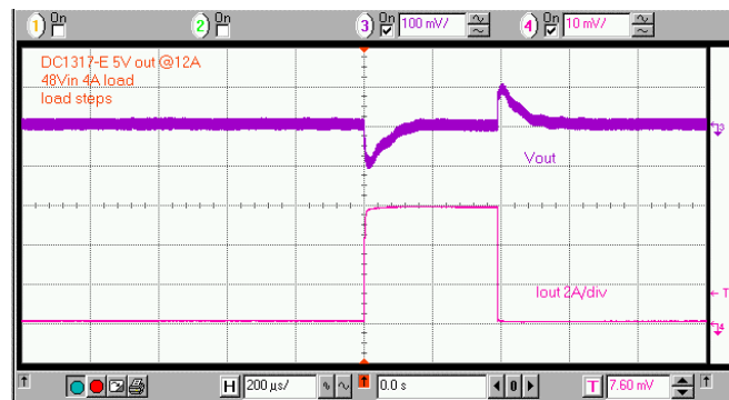
Figure 4. Fast transient response of DC1317A-E is superior to many competing power modules without the additional output capacitors.
