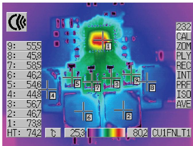
Figure 2. Thermal Image at V_{IN} = 12\text{V} , f = 1\text{MHz} with All Channels Sourcing 1A Current
