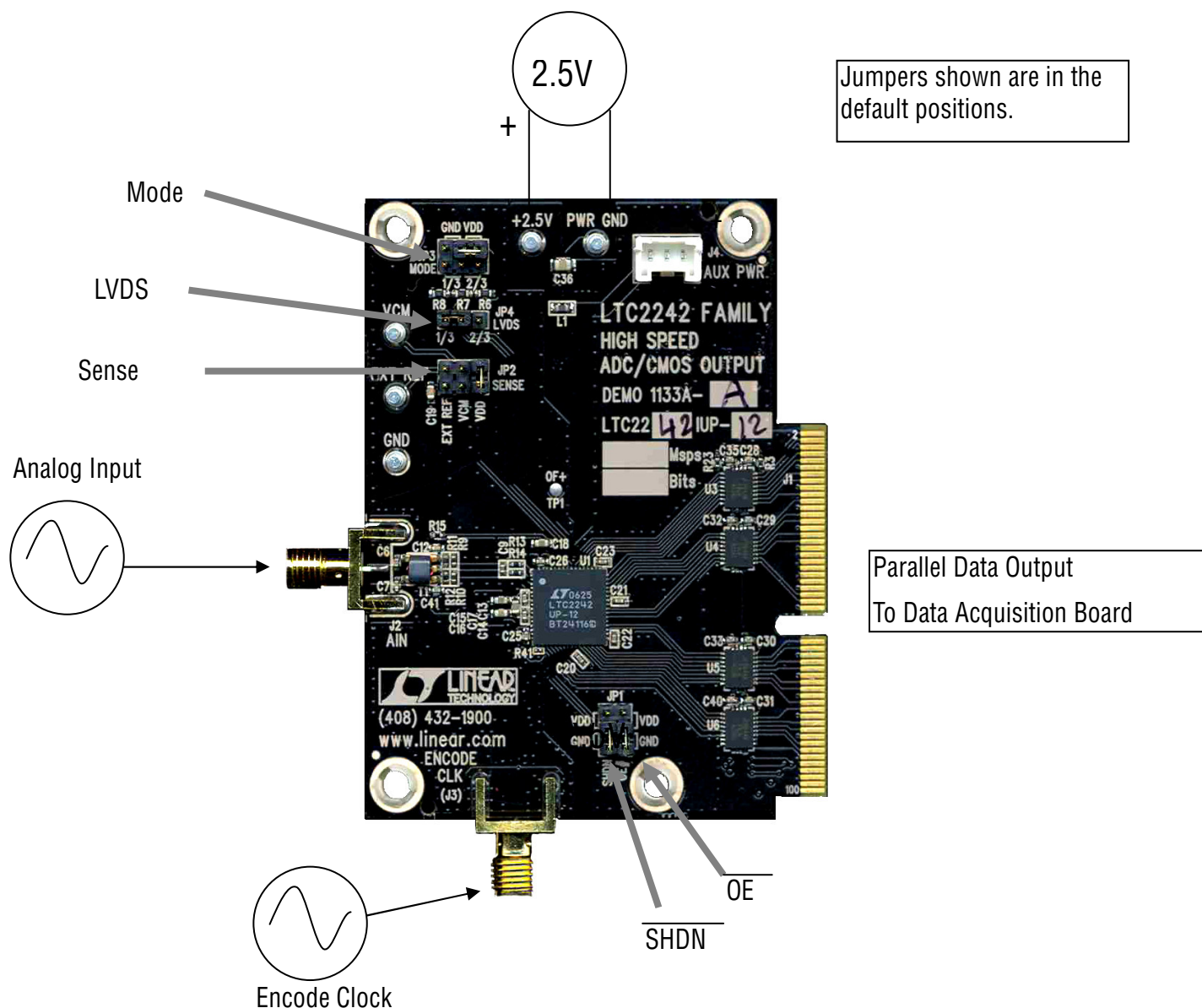
Figure 1. DC1133 Setup
