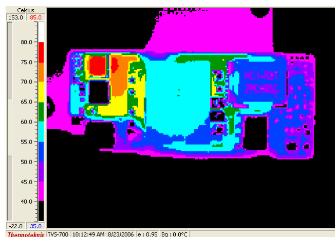
Figure 8. Temp Data (36Vin, 20A, 25°C, 200LFM airflow – front)
