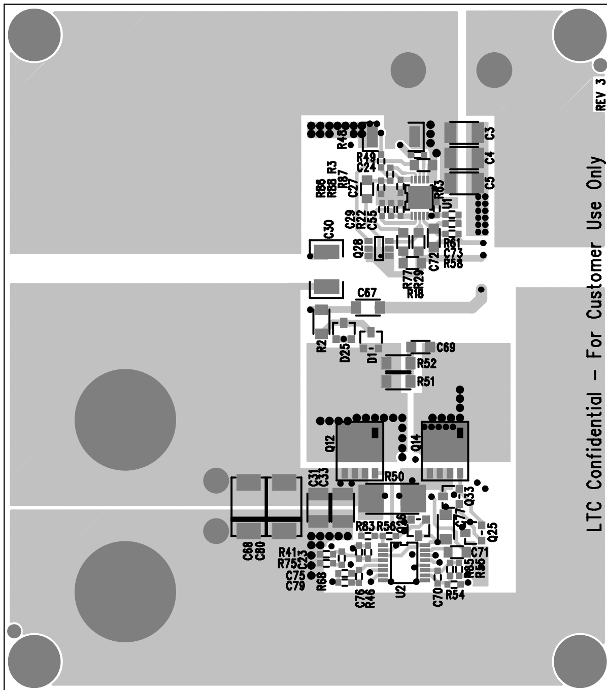
Figure 21. Bottom Mirrored
