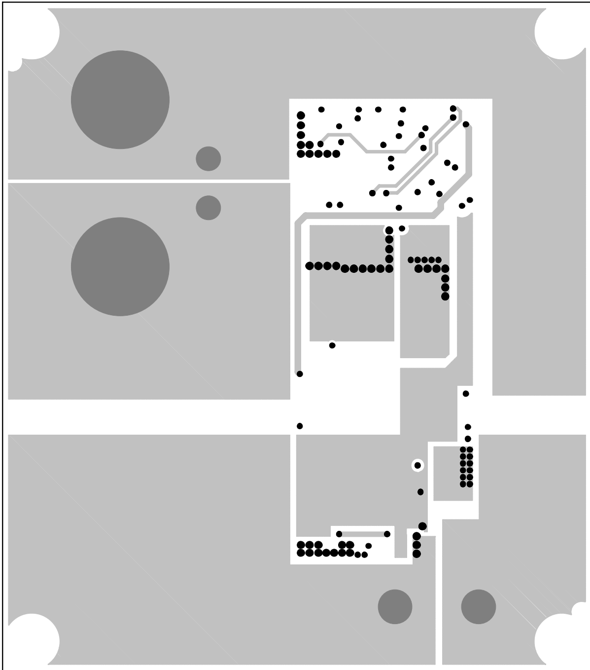
Figure 17. Layer 3
