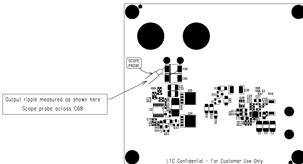
Figure 2. Measuring Input or Output Ripple
