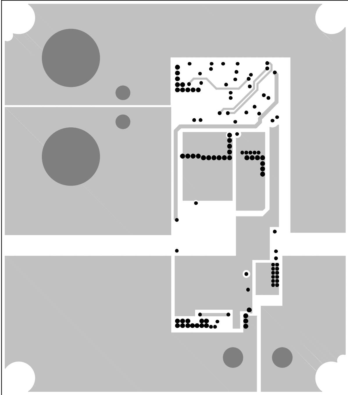
Figure 17. Layer 3
