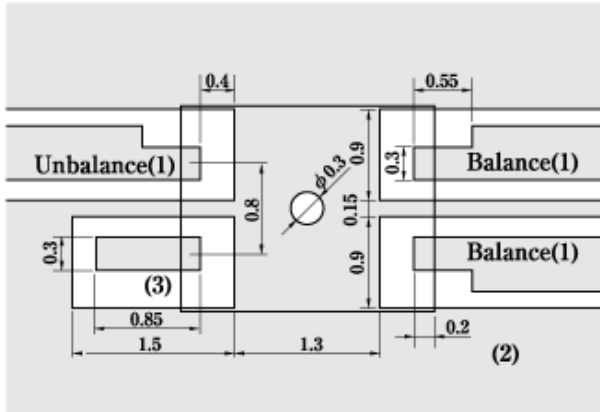
Land Pattern
