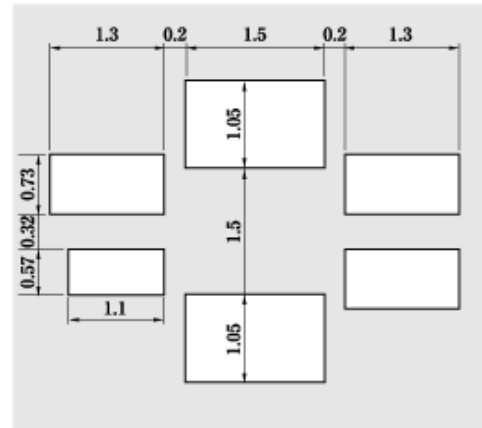
Resist Pattern
