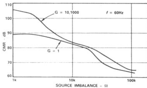
Figure 3. CMR vs Gain and Source Imbalance DAS1155/DAS1156
