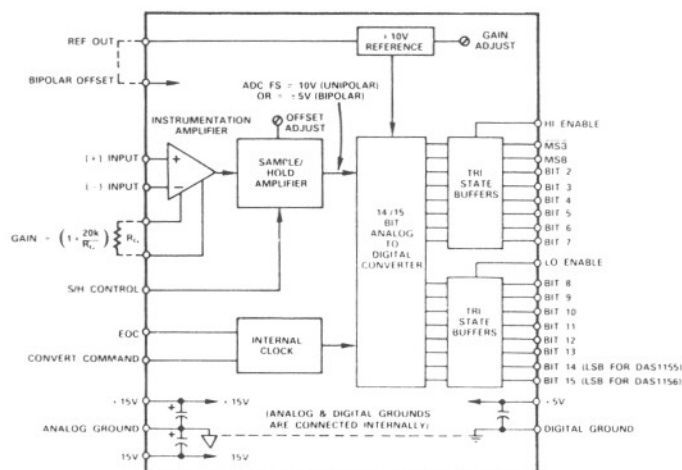
Figure 1. DAS1155/DAS1156 Block Diagram
