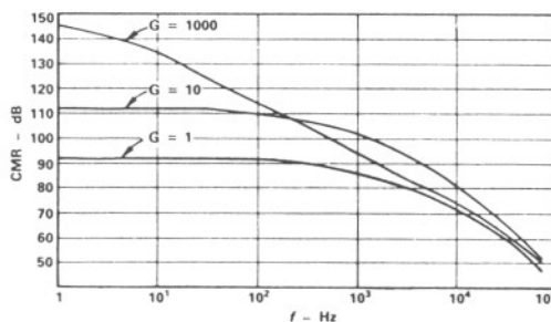
Figure 4. CMR vs Frequency DAS1155/DAS1156
