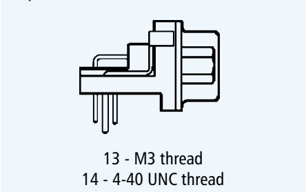
Jackpost
