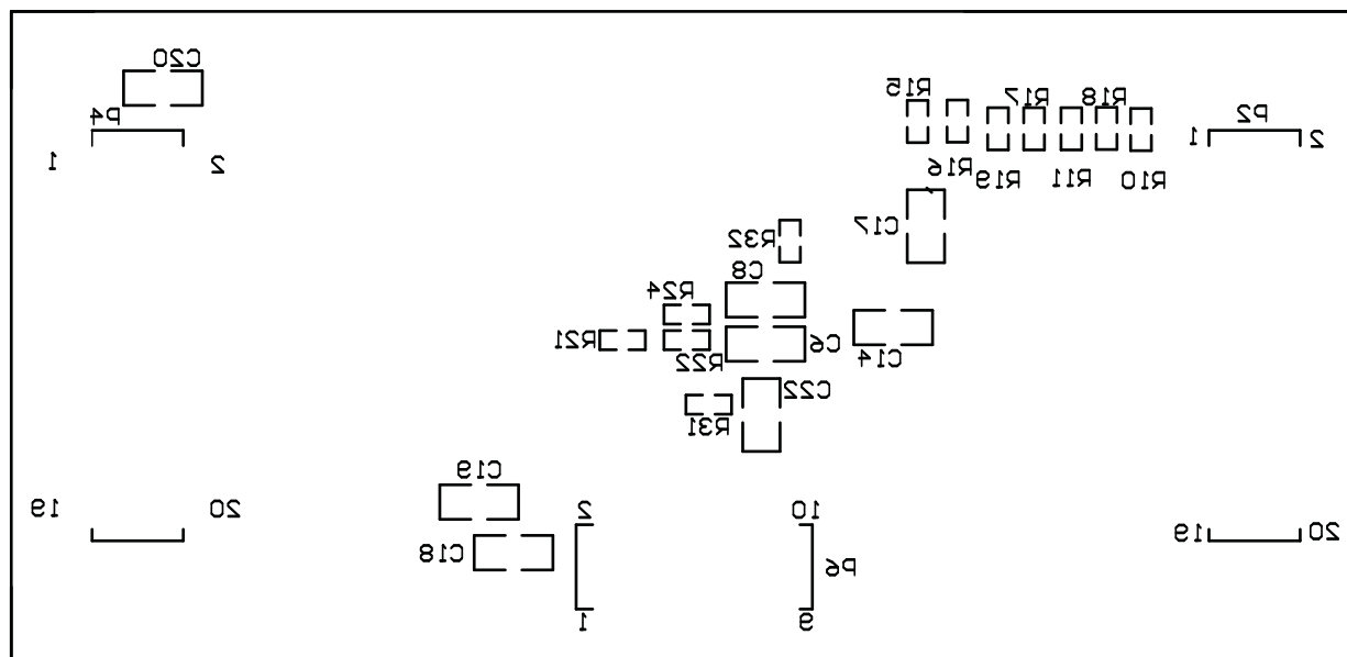
Figure 7. Bottom Silkscreen
