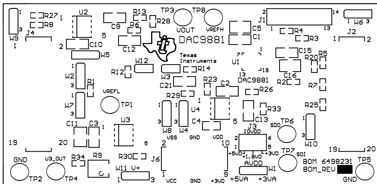
Figure 2. Top Silkscreen
