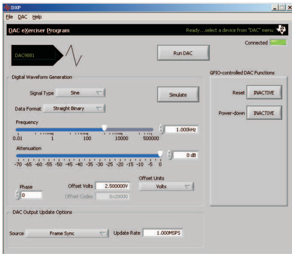
Figure 12. DAC9881 – Frequency/Amplitude and GPIO Control Options
