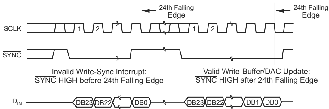
Figure 34. Interrupt and Valid \overline{\text{SYNC}} Timing
