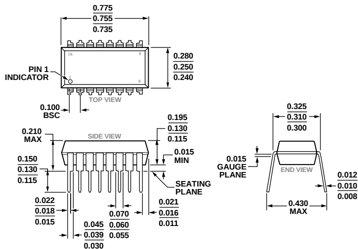
Figure 38. 16-Lead Plastic Dual In-Line Package [PDIP]
