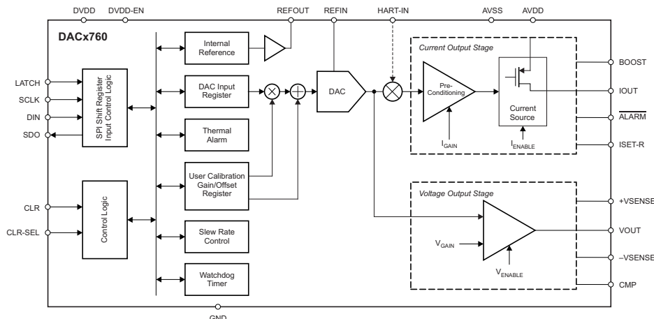
Block Diagram
