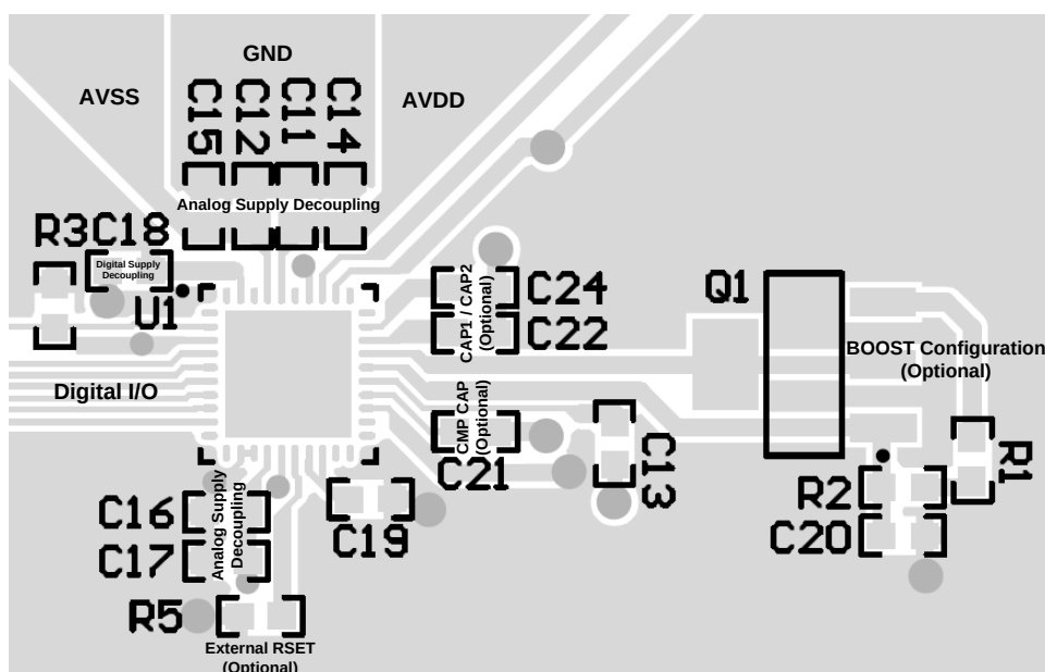
Figure 65. Example Layout
