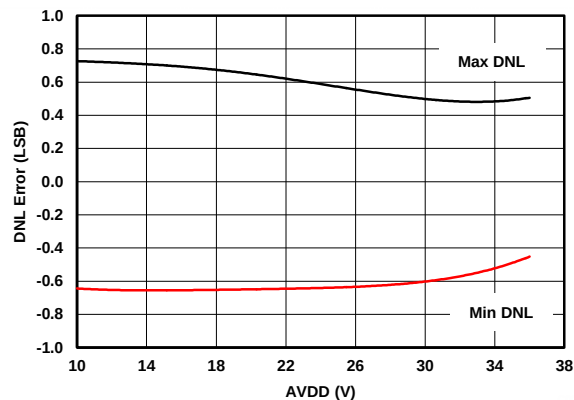
Figure 35. IOU DNL vs Supply (External R_{SET} )
