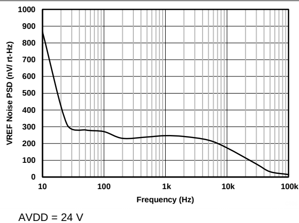
Figure 8. REFOUT Noise PSD vs Frequency
