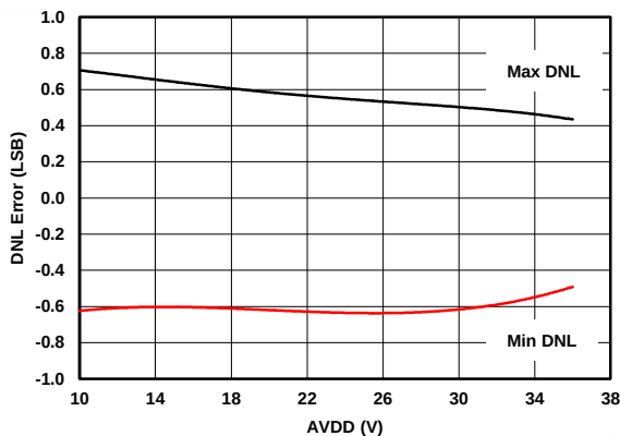
Figure 34. IOU DNL vs Supply (Internal R_{SET} )
