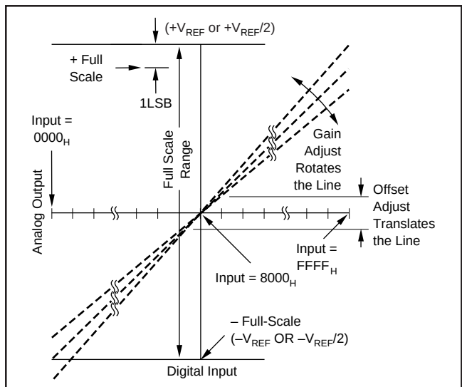
FIGURE 10. Relationship of Offset and Gain Adjustments for V_{OUT} = -10V to +10V Output Configuration. (Same Theory Applies for V_{OUT} = -5V to +5V .)
