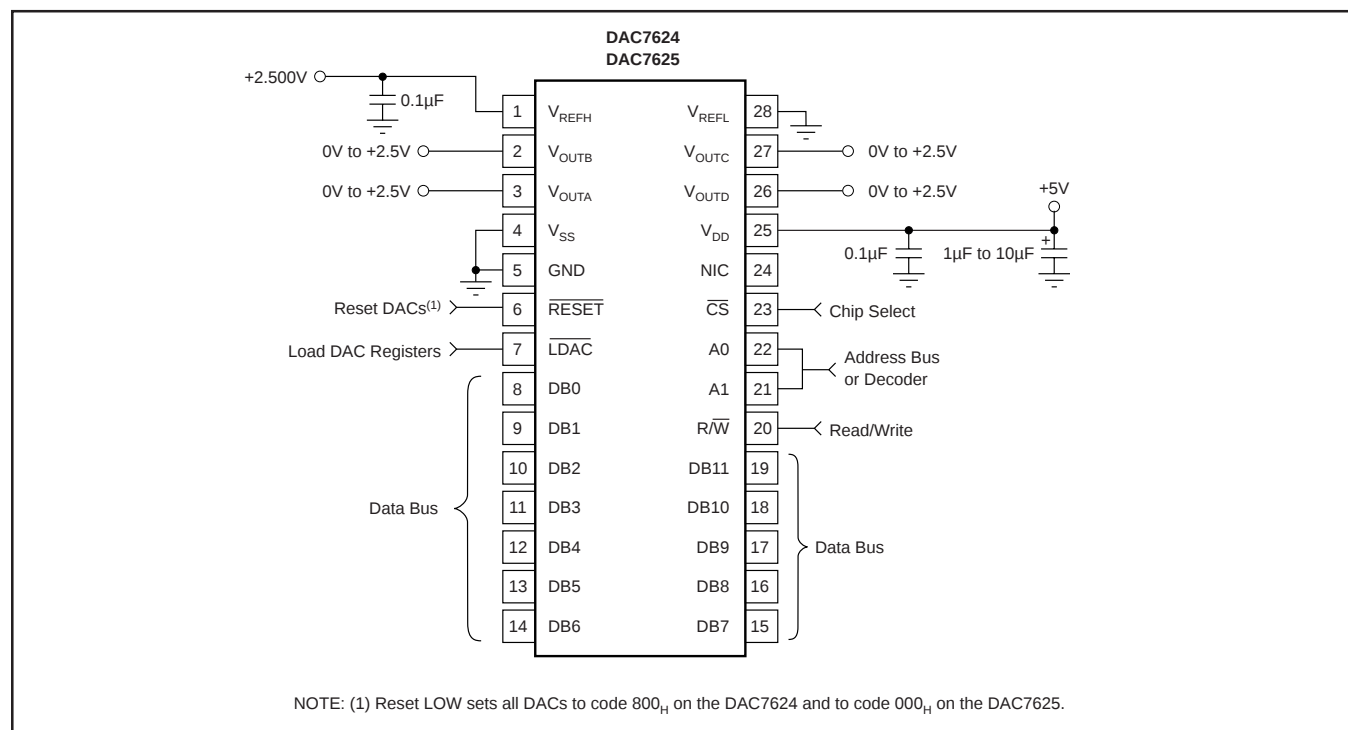
FIGURE 1. Basic Single-Supply Operation of the DAC7624/25.
