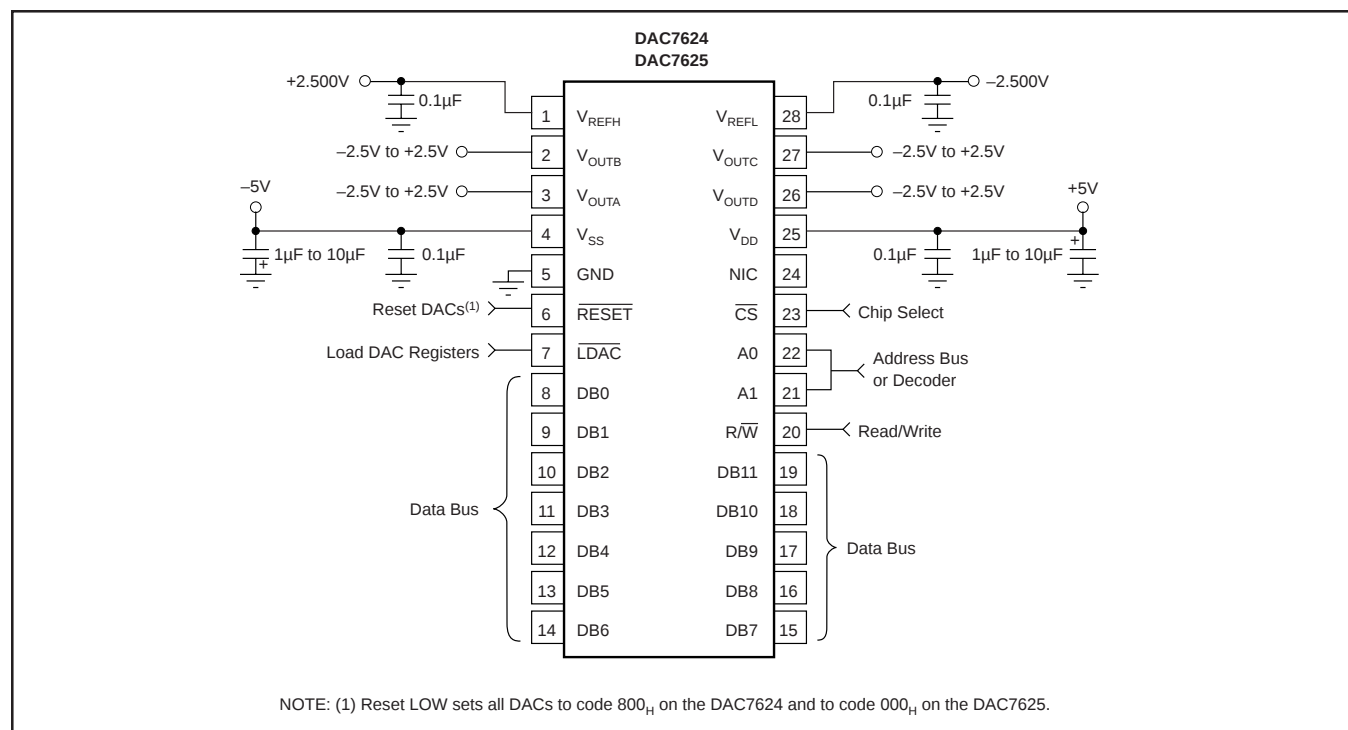
FIGURE 2. Basic Dual-Supply Operation of the DAC7624/25.
