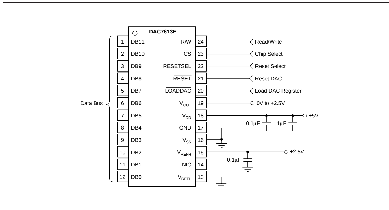
FIGURE 1. Basic Single-Supply Operation of the DAC7613.
