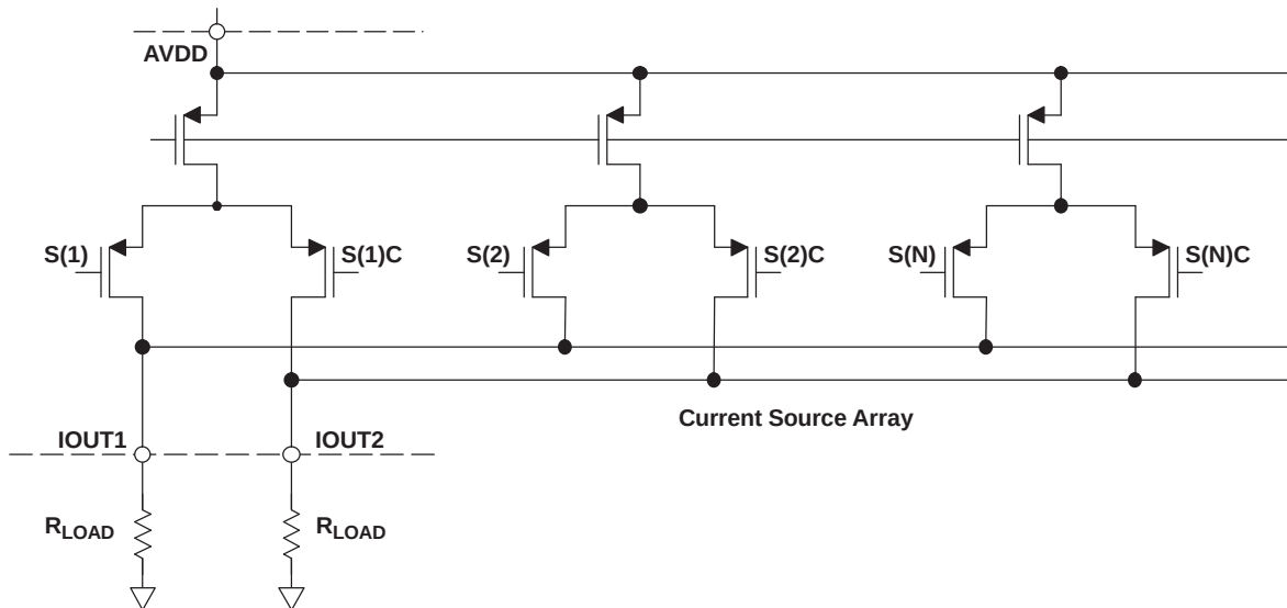
Figure 17. Analog Outputs
