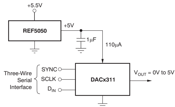
Figure 91. REF5050 as Power Supply to DACx311
