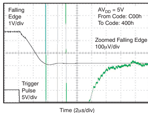
Figure 33. Half-Scale Settling Time 5-V Falling Edge
