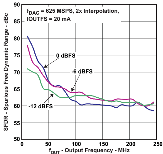
Figure 3. SFDR vs Input Scale
