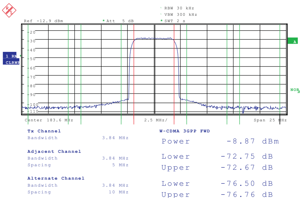
Figure 10. WCDMA ACPR (DAC Ch. B): DAC Clk = 614.4 MHz, 2× Int, f_s/4 Mixing, 30-MHz Offset; 183.6-MHz IF
