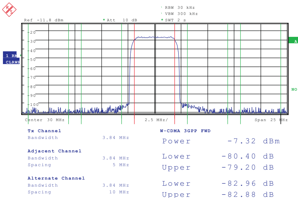
Figure 9. WCDMA ACPR (DAC Ch. B): DAC Clk = 614.4 MHz, 2× Int, 30-MHz Offset
