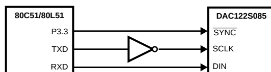
Figure 37. 80C51/80L51 Interface
