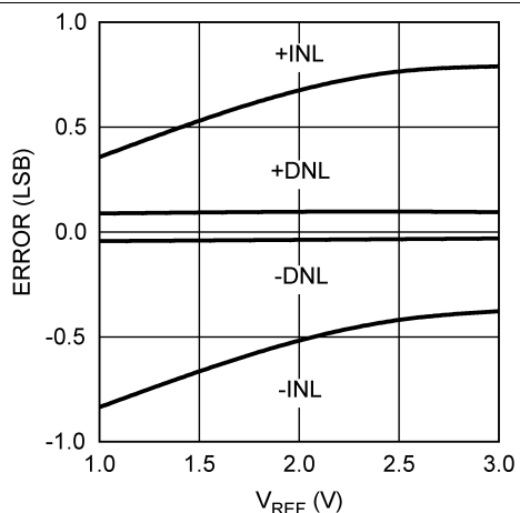
Figure 6. INL/DNL vs V_{REF} at V_A = 3 V
