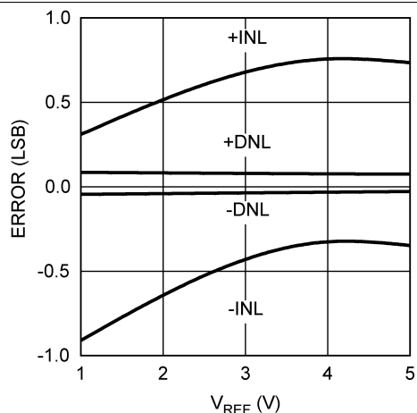
Figure 7. INL/DNL vs V_{REF} at V_A = 5 V
