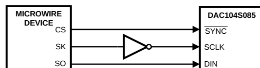
Figure 32. Microwire Interface
