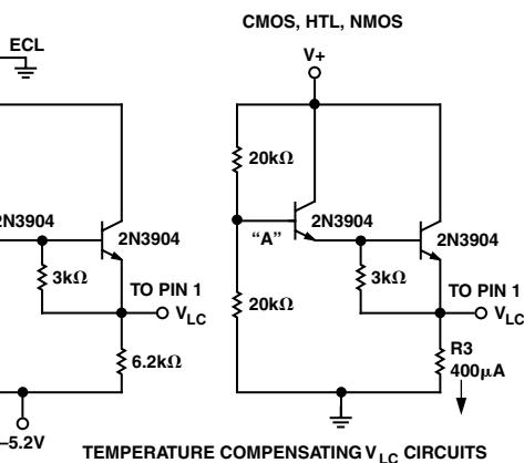
Figure 16. Interfacing with Various Logic Families
