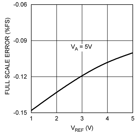
Figure 21. Full-Scale Error vs V_{REF}
