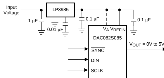
Figure 39. Using the LP3985 Regulator
