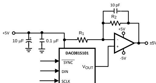
Figure 45. Bipolar Operation
